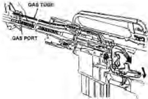
Figure 2-6. Firing.
