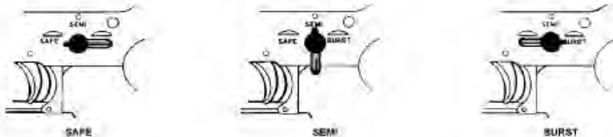
Figure 2-3. Selector Lever.
